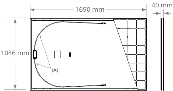
FRAME PROFILE
